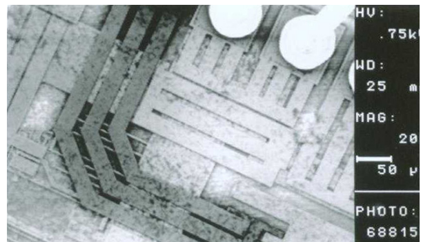
Low potential is visualised by voltage contrast. Dark conductor has low potential.
