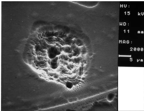
ESD failure on a FET observed by scanning electron microscopy after deprocess of the die (enlargement is 2000X).
