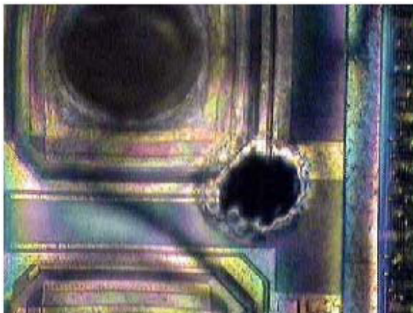
Location of degraded protection circuit by use of hot spot analysis.
