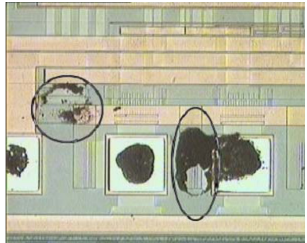
Removal of encapsulation material reveals carbonised material at two areas associated with data pins. Failure sites are located.
