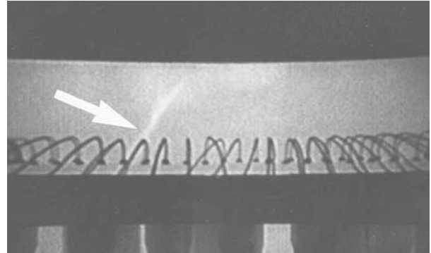
Void and microcrack encapsulation defects detected by non-destructive real time X-ray examination.
