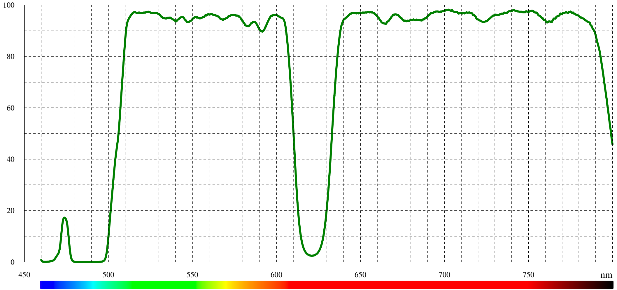
Typical transmission for MDCLP 505, 635 (LF101800)
