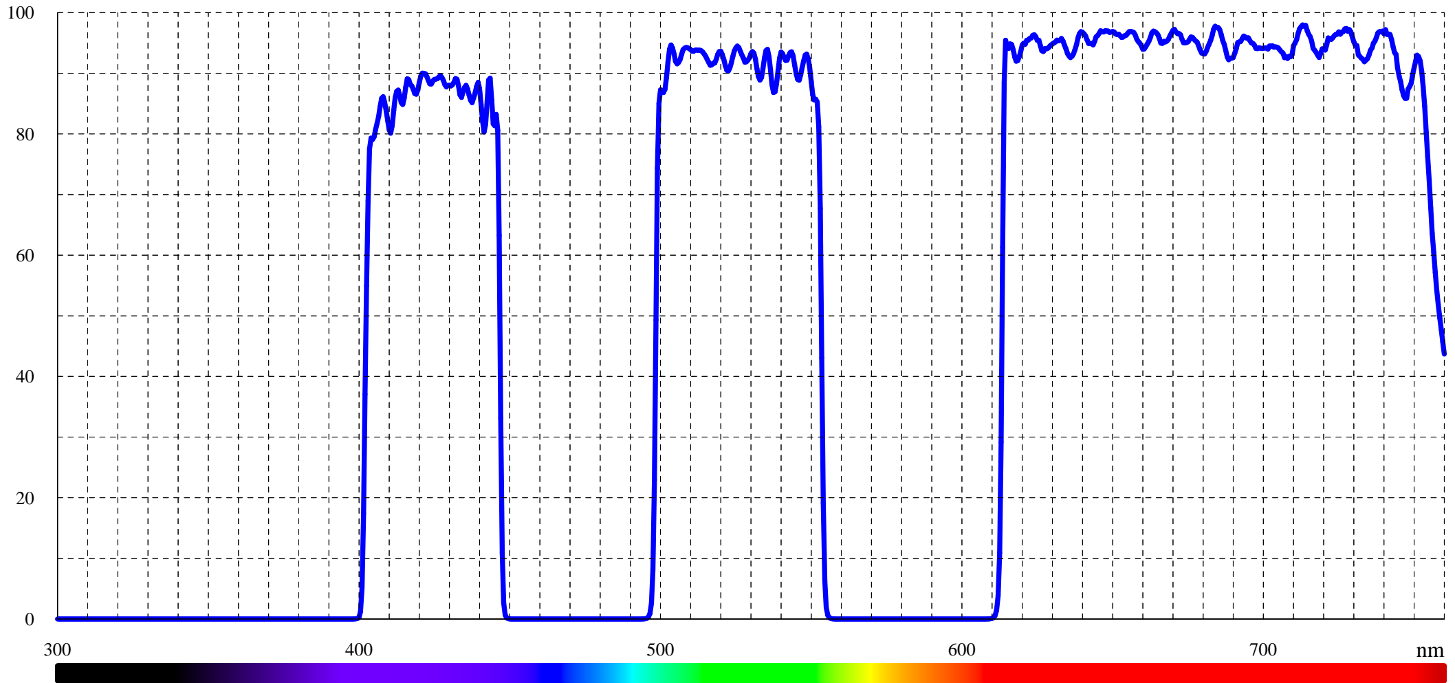
Typical transmission of MBP 425, 527, 685 (LF101810)
