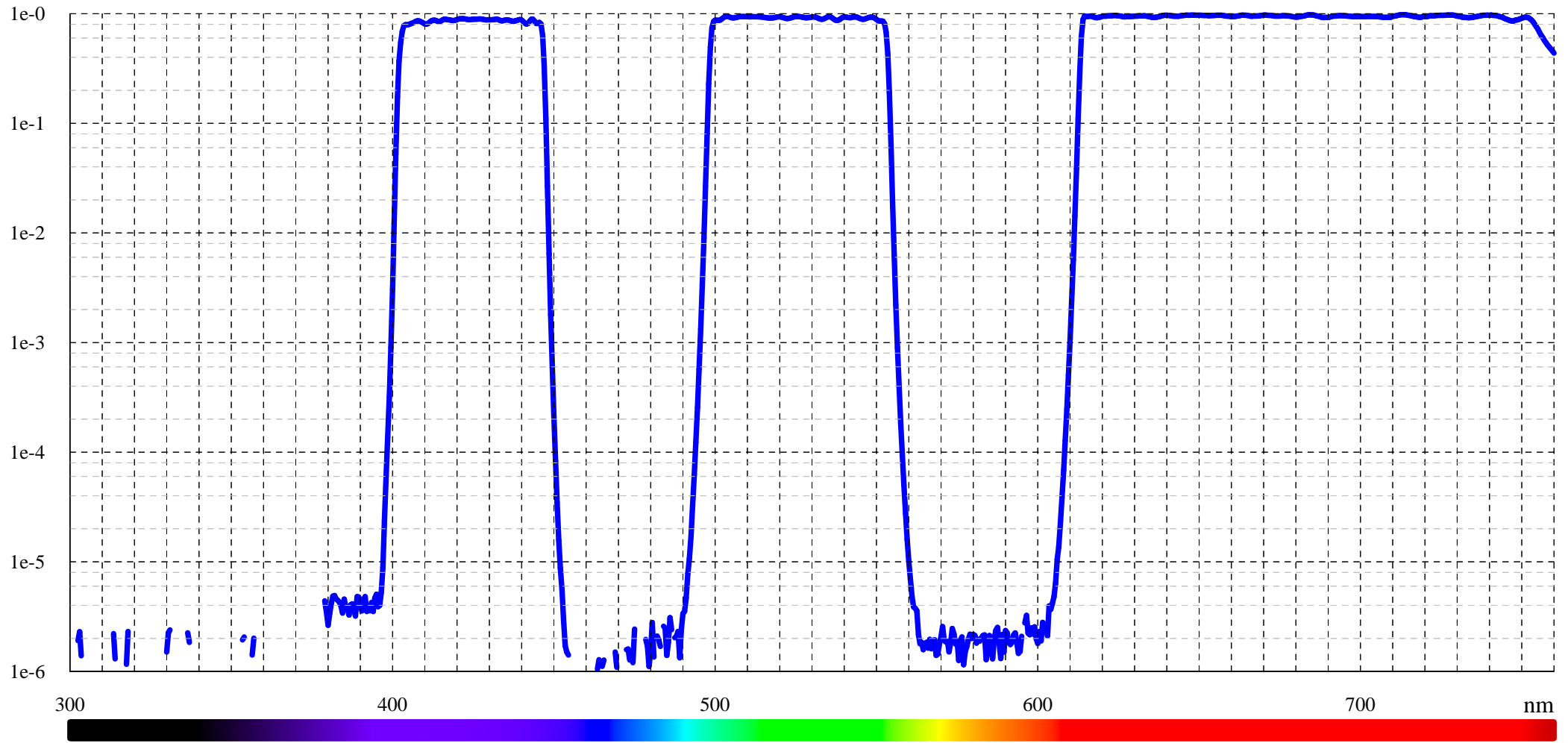
Typical blocking of MBP 425, 527, 685 (LF101810)
