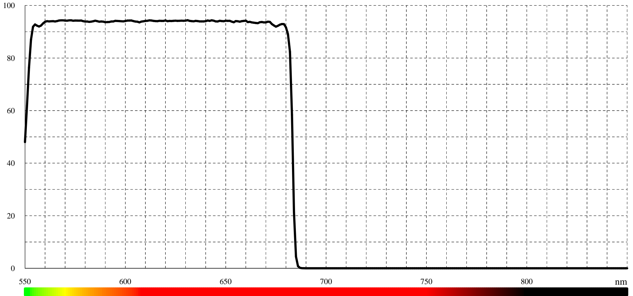
Typical transmission for SP682 (LF101855)
