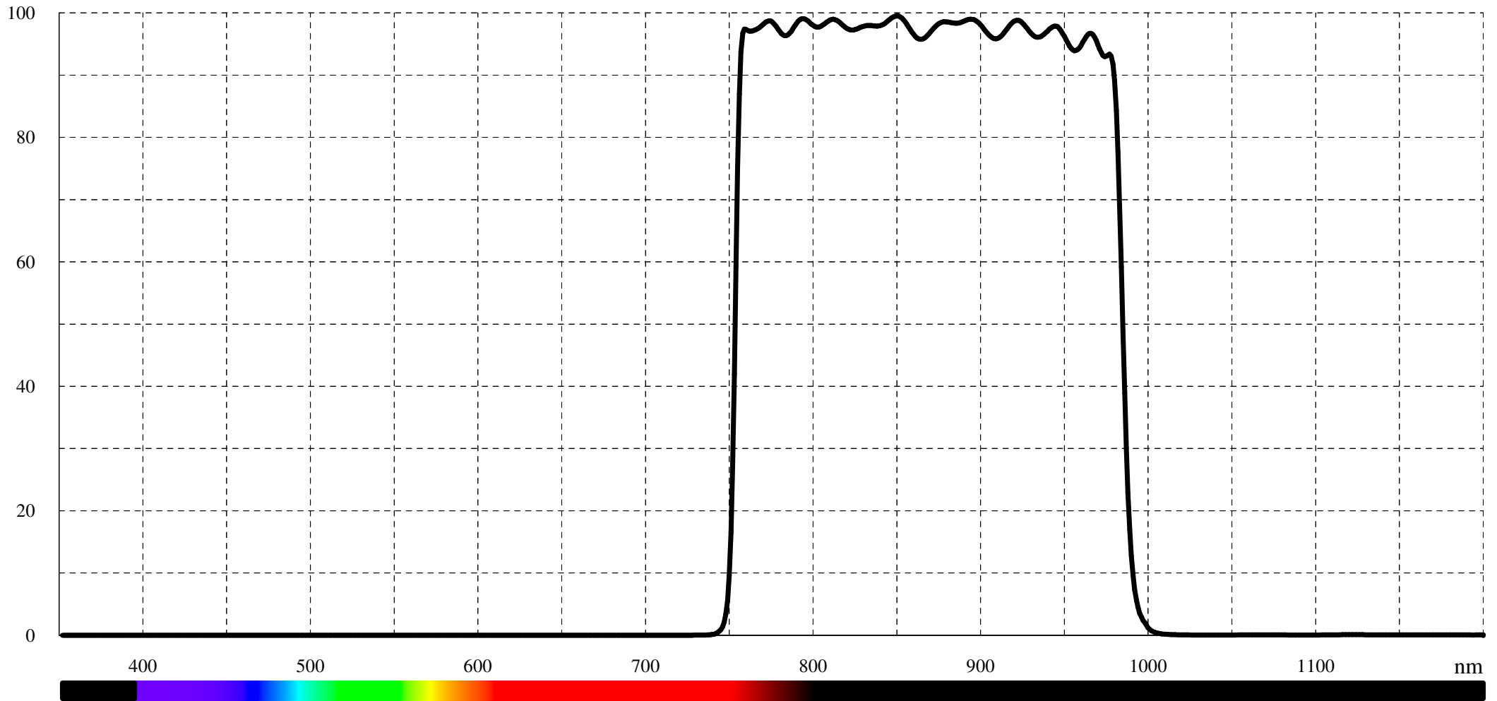
Typical transmission for BP 870/240 (LF101730)
